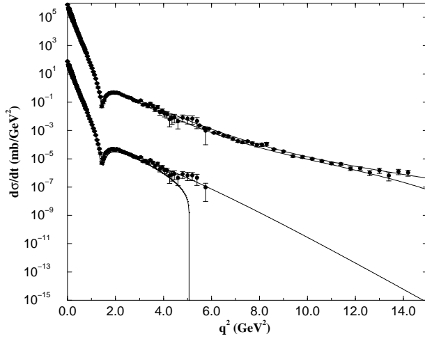
Figure 7. Regions of uncertainties (limited by the solid lines) in fits to pp differential cross section data, Eq. (23), at \sqrt{s} = 23.5 GeV with ensembles I (below) and II (above) [23].
