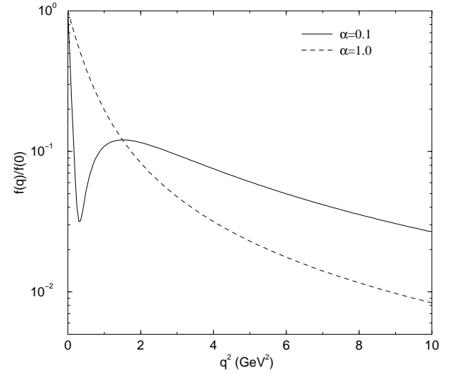
Figure 17. Elementary amplitudes from the constrained instanton approach.
