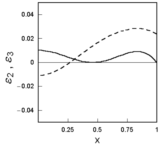
Figure 4. Slip factors \varepsilon_2 (filled line) and \varepsilon_3 (dashed line) as functions of x = r/a , for the case \lambda=1000 , \delta=0.227 , h = \sqrt{2} and C=0.3 (screw pinch case).
