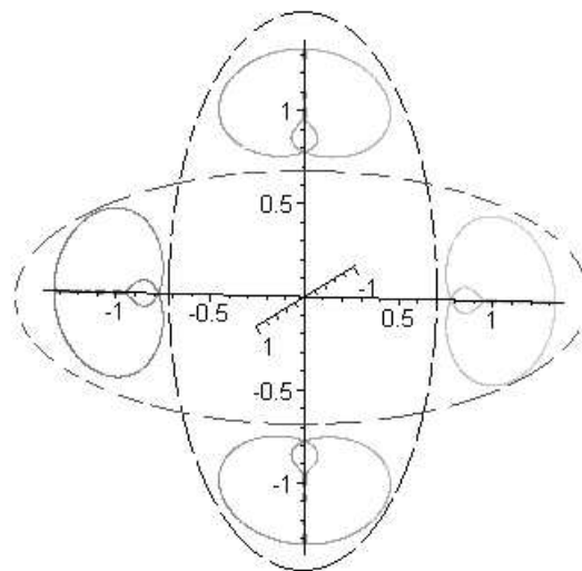
Figure 3. Distinct attractors (divide by traceable lines) with Klein symmetry preserved.
