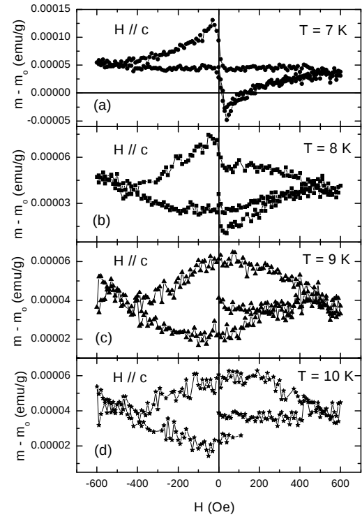
Figure 2. Zero-field-cooled magnetic moment hysteresis loops m(H) , after the subtraction of the diamagnetic background signal ( m_o = \chi H , where \chi = -7.12 \times 10^{-6} emu g ^{-1} Oe ^{-1} ), with H \parallel c and for (a) T = 7 K, (b) T = 8 K, (c) T = 9 K and (d) T = 10 K (the last part of this hysteresis loop was not measured). For details see text.
