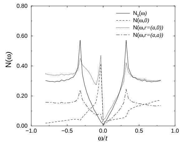
Figure 4. Density of states for a non-magnetic impurity in a DDW state: full line: d-wave gap without impurity, dashed line: at the impurity site, dotted line: at the nearest neighboring site along the x-axis, dotted-dashed line: at the nearest neighboring site along the diagonal of the crystal lattice.
