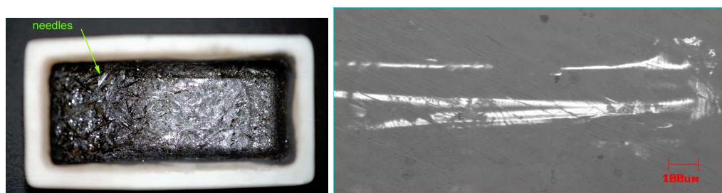
Figure 2. (a) Alumina crucible with needle-shaped single crystals no extracted (b) needle extracted from batch C4.
