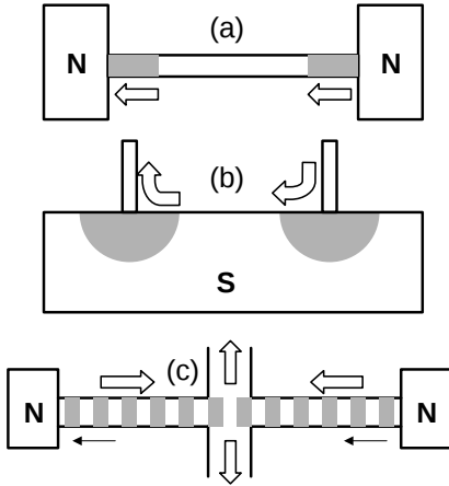
Figure 4. Geometries in which the interband phase breakdown could occur. Here N labels normal electrodes, gray domains show phase solitons moving along thin arrows, and block arrows indicate current directions. Static phase textures form in microbridges (a) and point contacts (b), while in the four-terminal geometry (c) the solitons and antisolitons continuously annihilate in the center.
