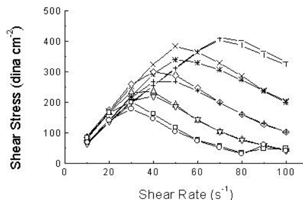
Figure 3. Rheograms of the LK/KCl/DeOH/H 2 O system : — 5 th shearing (25.0°C); -|- 6 th shearing (25.0°C); -* 8 th shearing (22.5°C); -◇- 9 th shearing (20.0°C); -+- 10 th shearing (20.0°C); -△- 11 th shearing (17.5°C); -▽- 12 th shearing (17.5°C); -□- 13 th shearing (15.0°C); -○- 14 th shearing (15.0°C) [64].
