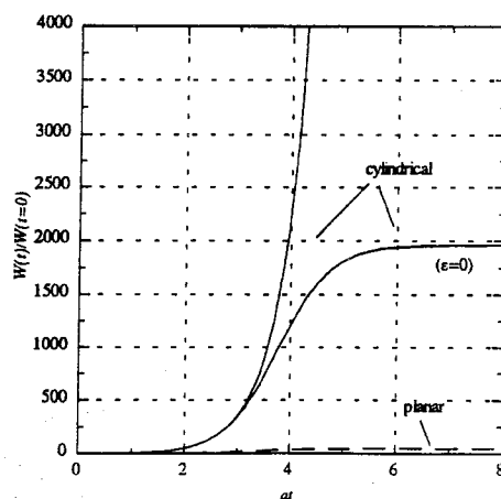
Fig. 24. Magnetic energy evolution in the PF.
