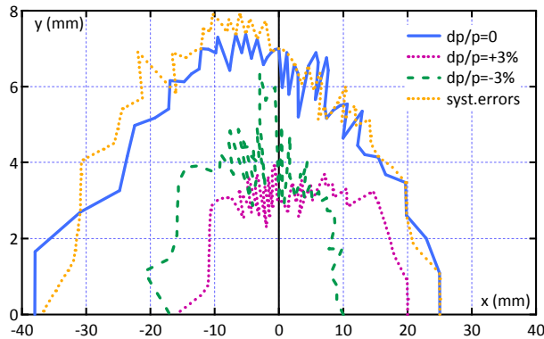
Figure 5: Dynamic aperture tracking for 4096 turns in the middle of the long SS ( \beta_x=28.7\text{m} , \beta_y=2.4\text{m} ) with MAD.
