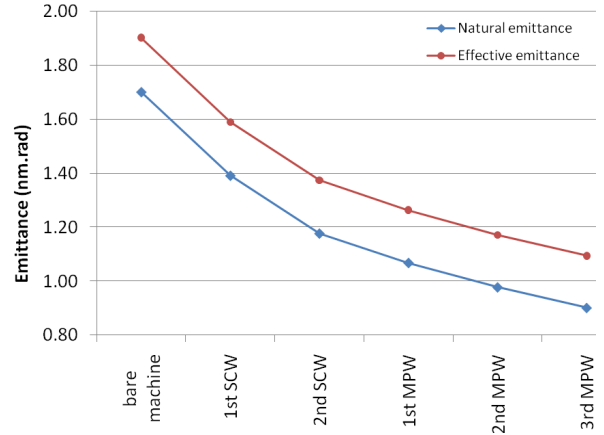
Figure 3: Evolution of natural and effective emittance as user IDs are installed in the ring. SCW is a 1 m, 4 T wiggler and MPW is a 2.7 m, 2 T wiggler.
