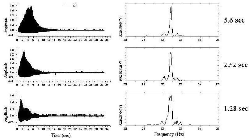
FIG. 5: Response to squared modulated pulses for various pulse-widths applied to the sample of 33 mg. The experiment is similar to what is done in Nuclear Magnetic Resonance.
