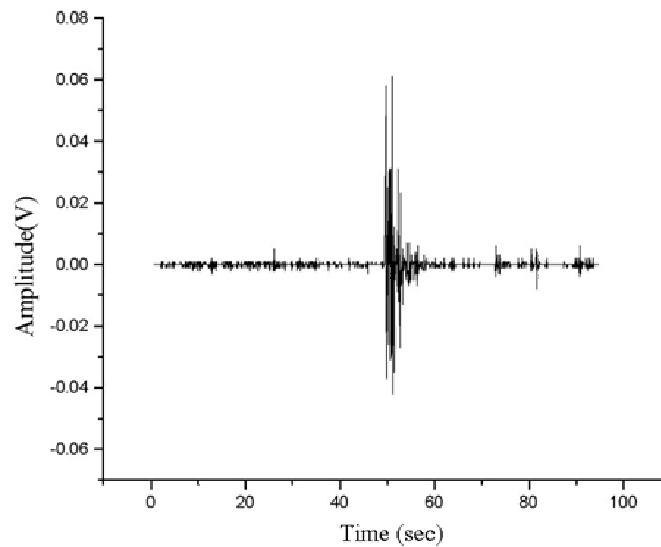
FIG. 6: Detection of mechanical noise in the workbench.
