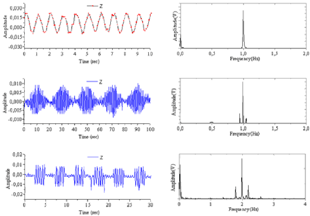
FIG. 3: (a) Response of the sensor to a single sinusoidal signal applied to an oscillating glass rod containing 33 mg of ferrite, and its Fourier transform. (b) and (c) Response to amplitude modulated signals, sinusoidal and square, respectively, and their Fourier transforms.
