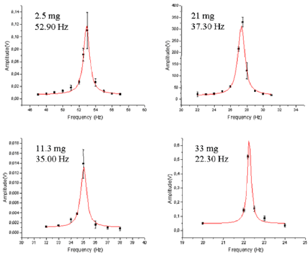
FIG. 4: Resonance curves, varying the excitation frequency point-by-point, for different masses of ferrite samples.
