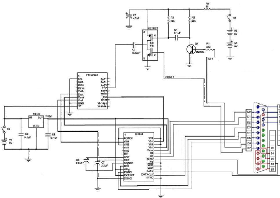
FIG. 1: Circuit board to communicate to the Honeywell HMC2003 sensor.
