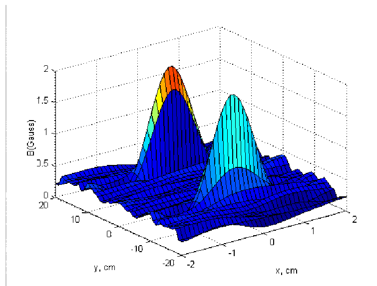
FIG. 2: Mapping of a static field around a solenoid with radius R = 1 cm and length L = 20 cm. The two peaks correspond to the edges of the solenoid. The region in between them was not mapped.
