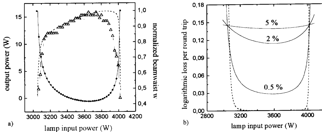
Figure 1. a) The solid dots represent the calculated, normalized beam waist versus lamp input power using equation (1) with w_0 = 0.42 mm, lower threshold P_1 = 3050 W and upper threshold P_2 = 4020 W. The straight line is an exact calculation of the beam waist using reference [1] and the data from the measured output power curve (triangles) is then fitted (dotted line) using equations (1) to (6) using 2% of heat conversion in the rod. b) diffraction losses (dotted line) and birefringence losses as a function of pump power percentage converted into heat.
