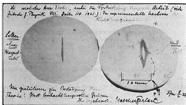
Gerlach's postcard, dated 8 February 1922, to Niels Bohr. It shows a photograph of the beam splitting, with the message, in translation: "Attached [is] the experimental proof of directional quantization. We congratulate [you] on the confirmation of your theory." (Physics Today December 2003)
