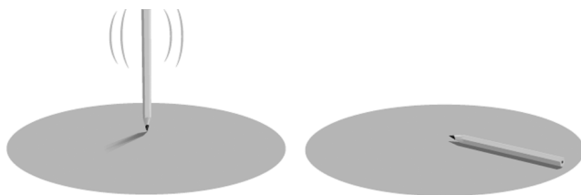
Figura 1 - Fonte: http://nobelprize.org/nobel_prizes/physics/laureates/2008/info.pdf .
