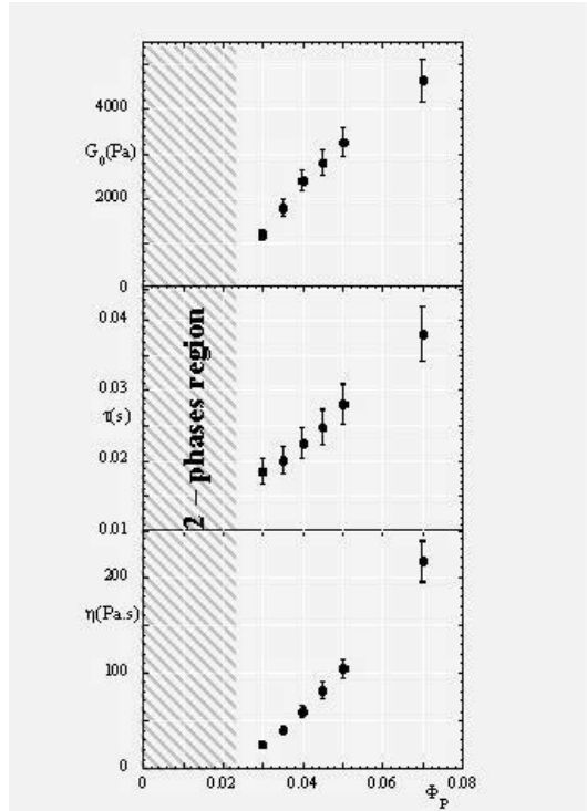
FIG. 3: Modulus G in Pa, \tau in s and \eta in Pa.s of 35k copolymer network as a function of polymer volume fraction \Phi_p .
