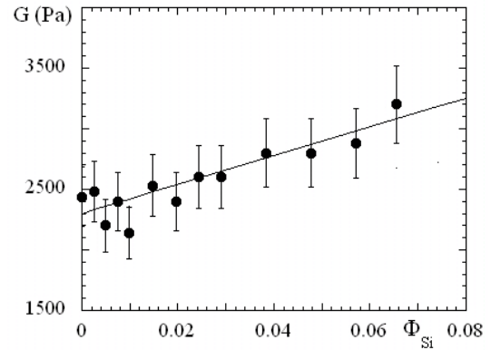
FIG. 4: Modulus G in Pa of filled 35k copolymer network ( \Phi_p = 3\% ) for increasing silica volume fraction \Phi_{Si} . All samples are at pH 10.
