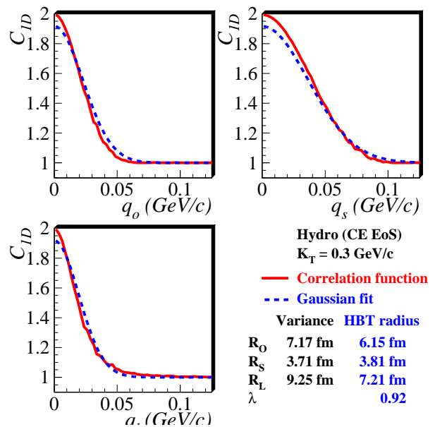
FIG. 10: (Color online) Solid (red) curves show one-dimensional slices of the three-dimensional correlation function calculated with Eq. (3) from the hydrodynamic model with CE Equation of State, for midrapidity pions with K_T = 0.3 GeV/c. Dashed (blue) curves show slices of the three-dimensional Gaussian form of Equation (5), with “HBT parameters” calculated from the analytic expressions given in Sec. III B.
