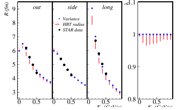
FIG. 9: (Color online) Three-dimensional HBT fit parameters R_{1D,i} and \lambda_{1D,i} as a function of K_T , calculated from the blast-wave parameterization with Eqs. (21). For a given K_T , the vertical red line represents the variation with fit range (see Fig. 8). Blue stars represent the corresponding radius parameters calculated from the RMS variances using Eq. (6). Black circles show STAR data [4], with error bars removed for clarity.
