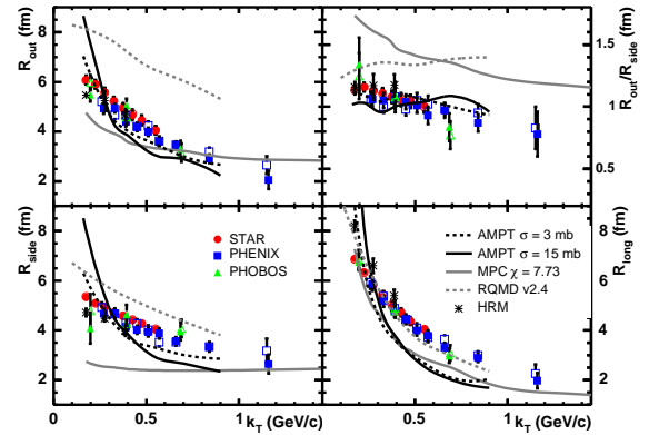
FIG. 3: (Color online) ‘‘HBT radii’’ calculated [17, 18, 20, 38] in Boltzmann-cascade models, compared to experimental radii extracted from fits. The calculated radii are discussed in the text. Compilation from [1].
