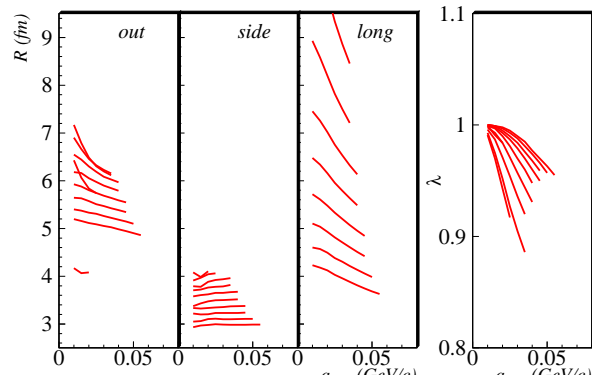
FIG. 11: (Color online) From the hydrodynamic model with CE EoS, three-dimensional HBT fit parameters R_i and \lambda are calculated with Eqs. (21) and plotted as a function of the maximum allowed value of any q -component; see text for details. Each curve corresponds to one of ten values of K_T : 0.0, 0.1, 0.2, ..., 0.9 GeV/c. Curves corresponding to high K_T are at low (high) values of R_i ( \lambda ). The R_i curves for K_T \leq 0.1 GeV/c fall above the plotting range.
