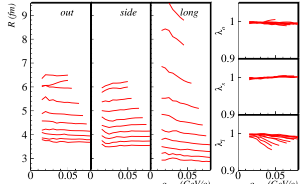
FIG. 6: (Color online) From the blast-wave parameterization, one-dimensional HBT fit parameters R_{ID,i} and \lambda_{ID,i} are calculated with Eqs. (13,14) and plotted as a function of the maximum allowed value of any q -component; see text for details. Each curve corresponds to one of ten values of K_T : 0.0, 0.1, 0.2, ..., 0.9 GeV/c. Curves corresponding to high K_T are at low (high) values of R_{ID,i} ( \lambda_{ID,i} ).
