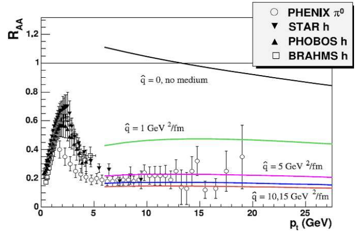
FIG. 2: Model fits to the nuclear modification ratio R_{AA} for \pi^0 mesons and charged hadrons in the BDMPS formalism, which fits the data as a function of a transport parameter \hat{q} . Note that because the suppression is so large, R_{AA} does not offer a great deal of discrimination over a wide range of \hat{q} . Figure from [8].
