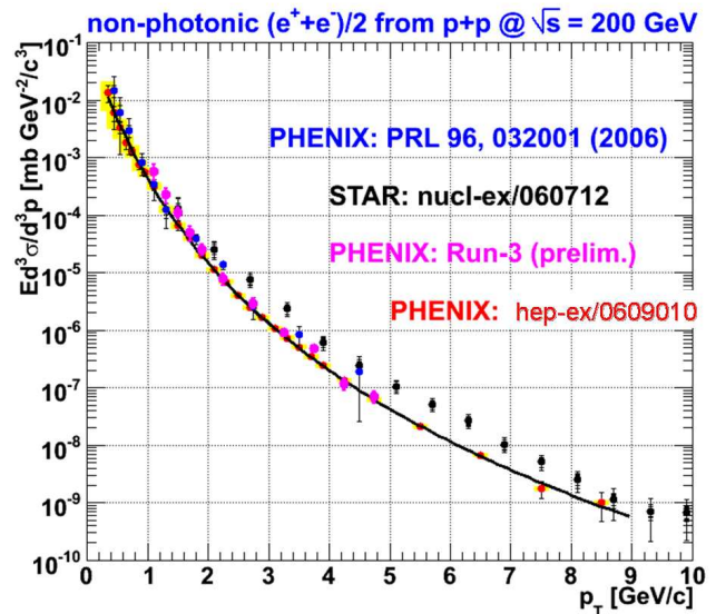
FIG. 4: The transverse momentum distribution of single inclusive electrons and positrons in proton-proton collisions, as measured by the STAR [16] and PHENIX [15, 18] collaborations. The multiple PHENIX datasets are in agreement with each other, within systematic and statistical errors. The line shown is a power-law fit to the most recent PHENIX data. Note that the recent STAR data are significantly higher than the PHENIX data at high- p_T .
