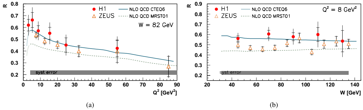
FIG. 1: (a) The skewing factor R as a function of Q^2 at W = 82 GeV [4]. The points correspond to the R extraction applied to DVCS measurements of H1 (bullets) and ZEUS (triangles). The curves represent R extracted from Freund et al. prediction based on MRST 2001 and CTEQ6 PDFs. (b) The skewing factor R as a function of W at Q^2 = 8 GeV 2 .
