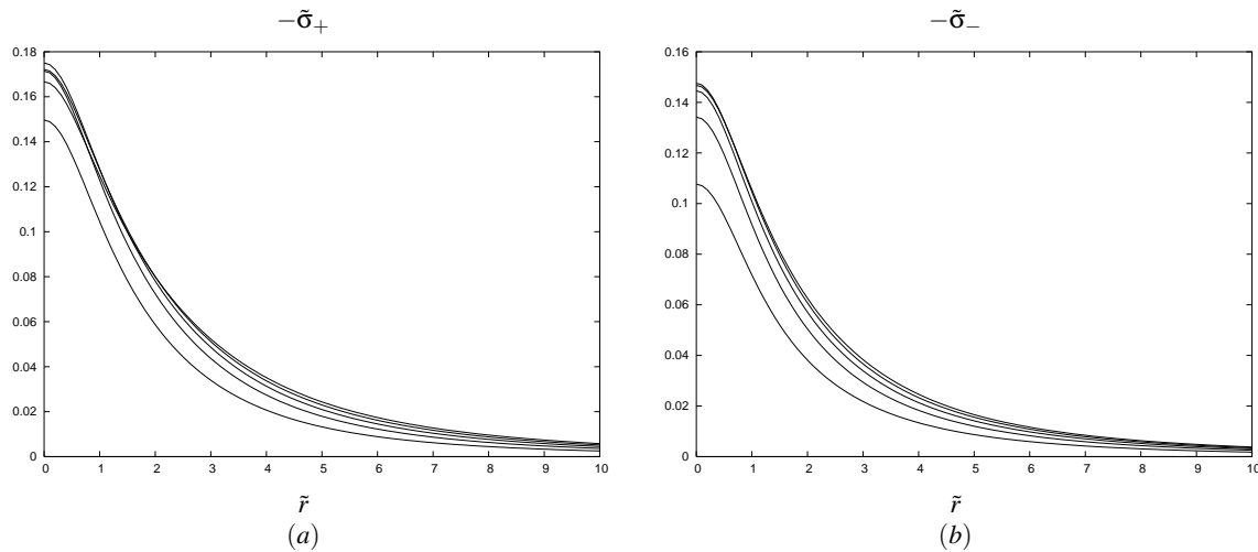
FIG. 7: The surface electric charge densities (a) \tilde{\sigma}_+ and (b) \tilde{\sigma}_- for electrogeodesic Kerr-Newman disks with \alpha = 2 , b = 0.2 and c = 1.0 (axis \tilde{r} ), 1.5, 2.0, 2.5, 3.0, and 3.5 (top curves away from the center of the disk), as functions of \tilde{r} .
