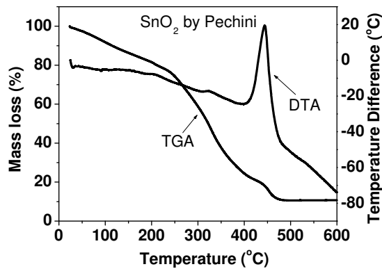
FIG. 5: TGA/DTA analysis for Pechini's SnO 2 .
