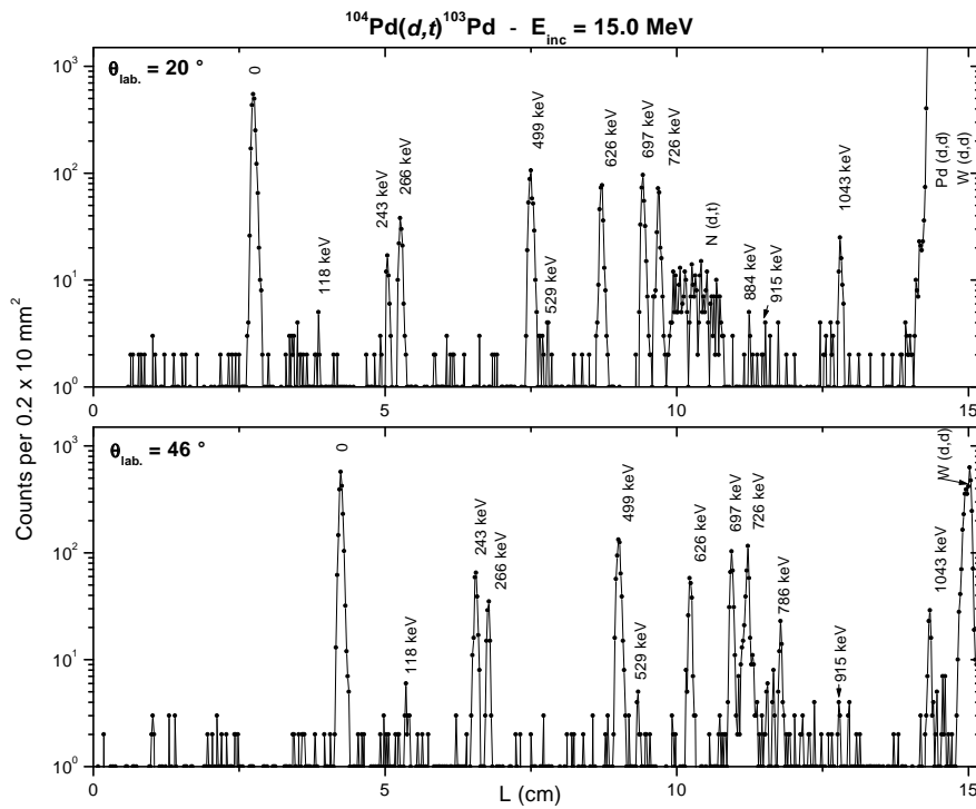
FIG. 1: Triton spectra obtained at 20^\circ and at 46^\circ laboratory scattering angles. The excitation energies attributed to the levels populated in the reaction are indicated above each of the corresponding triton peaks.
