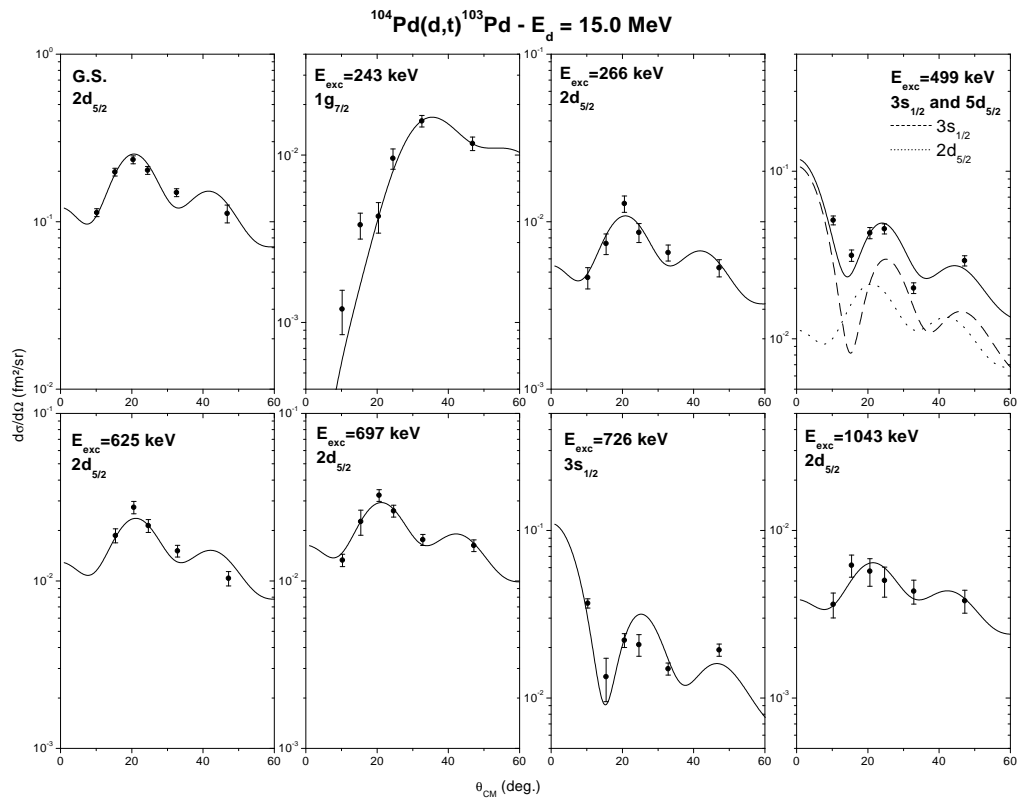
FIG. 2: Experimental angular distributions of ^{104}\text{Pd}(d,t)^{103}\text{Pd} in comparison with DWBA one-neutron pick-up predictions.
