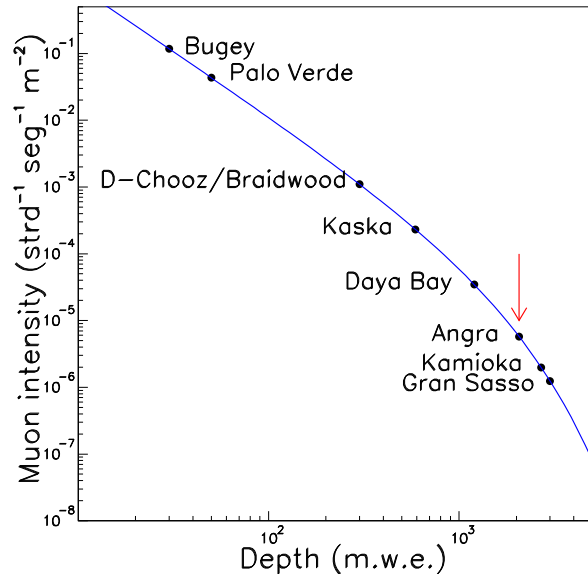
FIG. 2: The solid curves gives the underground muon flux extrapolated from the LVD experiment results [9]. Big dots indicate overburdens of different reactor experiments. The arrow points to the Angra FD situation. The two deepest installations, added for comparison purpose, are dedicated underground laboratories (Kamioka in Japan and Gran Sasso in Italy).
