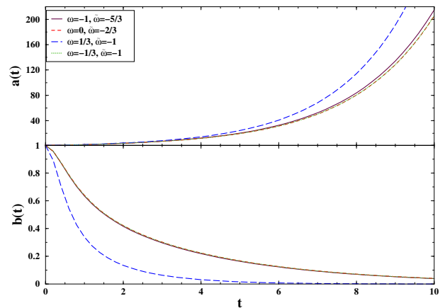
FIG. 2: Time evolution of the scale factors a(t) and b(t) for \Lambda_6 > 0 and k = -1 .
