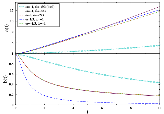
FIG. 4: Time evolution of the scale factors a(t) and b(t) for \Lambda_6 = 0 and k = 0, -1 .
