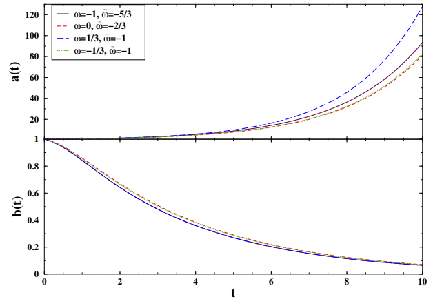
FIG. 1: Time evolution of the scale factors a(t) and b(t) for \Lambda_6 > 0 and k = 0 .
