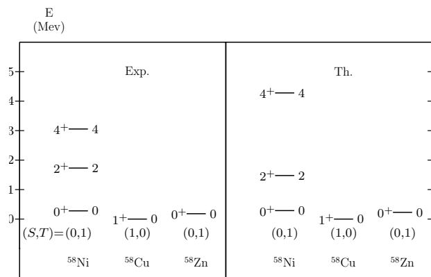
Figure 1. The spectra of the Ni-Cu-Zn nuclei with A=58 . The experimental energies are pure nuclear interactions, and the theoretical levels given by the SU(4) \otimes SU(6) model. For each level J^\pi (to the left) represents the total angular momentum and parity, and L (to the right) the orbital angular momentum. The spin-isospin number, (S, T) , are given for each nucleus.
