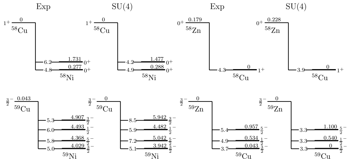
Figure 4. The beta decay of Ni-Cu-Zn isotopes with A=58 and A=59 .
