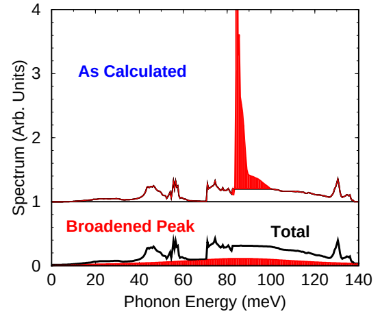
Figure 3. The upper panel shows the \alpha^2 F(\omega) spectral function that was calculated by An et al. [14, 13]. The lower panel shows the effect of broadening the contributions of the strongly coupled phonons (those within the peak near 85 meV) by a Lorentzian with a width equal to about 40% of the peak frequency ( \gamma=35 meV): notice that the peak vanishes. A proper theory would probably not give the simple Lorentzian broadening that arises in conventional Migdal-Eliashberg theory.
