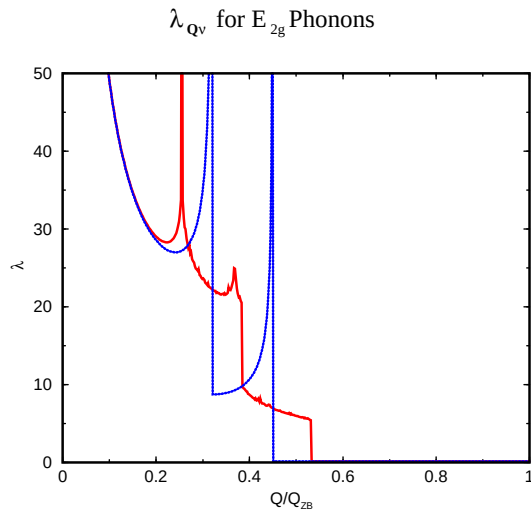
Figure 2. Behavior of \lambda_{Q_{||}} ( Q_{||} \equiv \sqrt{(Q_x^2 + Q_y^2)} ). The dotted line gives the behavior for two concentric 2D cylinder Fermi surfaces such as in \text{MgB}_2 , with (integrable) divergences at Q_{||} \rightarrow 0 as well as for Q_{||} = 2k_F for each of the two cylindrical Fermi surfaces. The full line shows the effect of k_z dispersion that is representative of \text{MgB}_2 .
