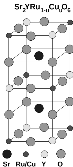
Figure 4. Crystal structure of \text{Sr}_2\text{YRu}_{1-u}\text{Cu}_u\text{O}_6 .
