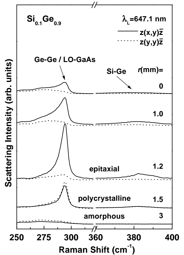
Figure 2. Raman spectra of a LC c\text{-Si}_{0.1}\text{Ge}_{0.9} alloy recorded at different radial distances r from the center of the LC spot. The fluencies for x = 0, 1, 1.2, 1.5, and 3 \text{ mm} are estimated to be 2000, 1250, 1000, 650, and 0 \text{ mJ/cm}^2 .
