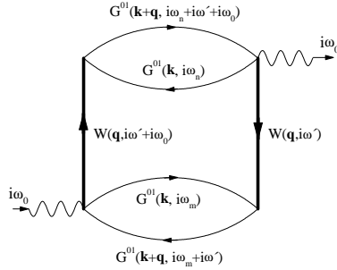
Figure 1. The Feynmann diagram for the drag resistivity.
