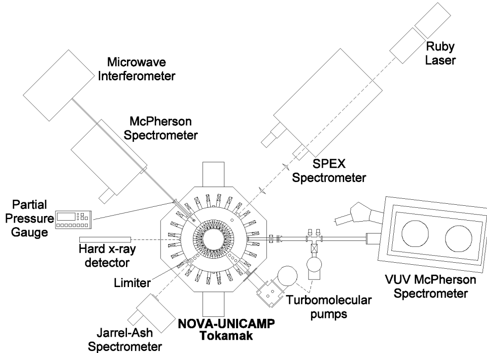
Figure 1. NOVA-UNICAMP tokamak and its main diagnostics.
