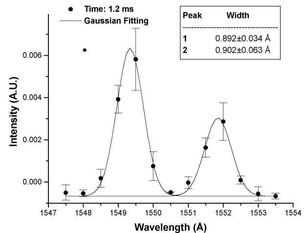
Figure 3. Top: Overlapping of CIII and OII four emission spectra in visible region; notice Doppler broadening deviation for each spectra giving different temperatures for same species. Bottom: VUV spectra of CIV emission; notice very well defined Doppler broadening for both emissions.
