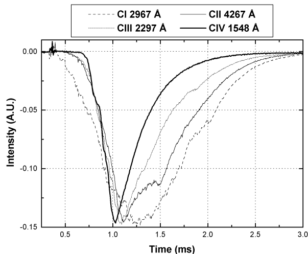
Figure 8. Different ionized carbon emissions (zoom).
