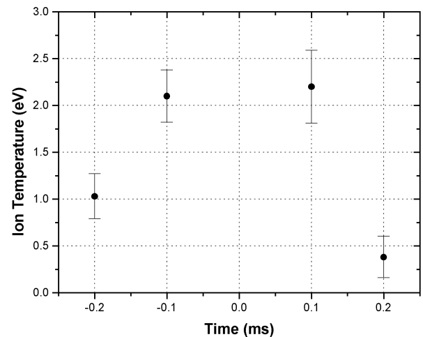
Figure 9. HeI temperature in low energy discharge.
