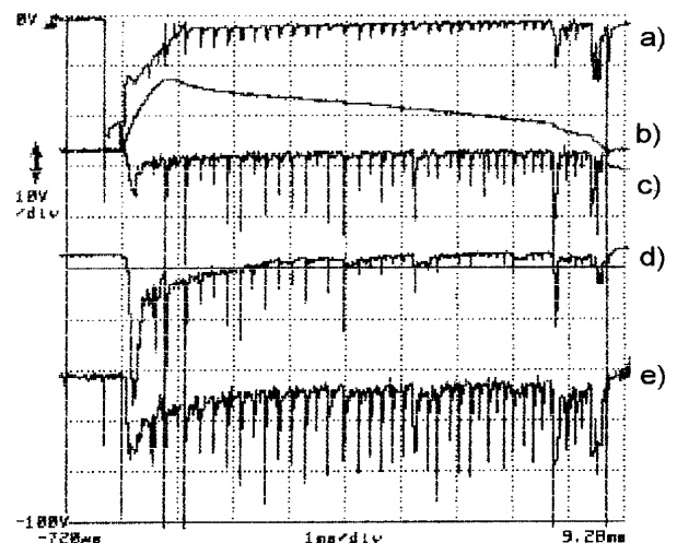
Figure 4. Oscillations of 2 kHz peaks, in loop voltage and spectral line signals at three toroidal positions: a) Loop Voltage; b) Plasma Current; c) H_{\alpha}-0^0 ; d) H_{\alpha}-90^0 ; e) H_{\alpha}-180^0 .
