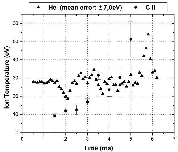
Figure 6. HeI (helium plasma) and CIII (hydrogen plasma) ion temperature.
