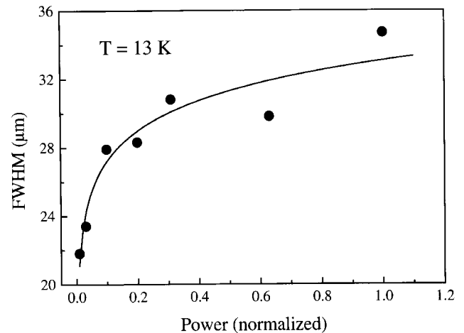
Figure 4. Spatial PL distribution (FWHM) at 13 K as a function of the excitation intensity. The solid line is only to guide the eyes.
