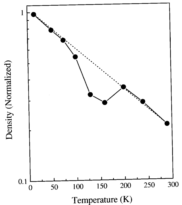
Figure 3. Total carrier density that recombine radiatively as function of temperature. We observe an abrupt change on the carrier density at about 150 K, which may be associated to thermal activation of an impurity related recombination channel. The solid and dashed lines are only guides to the eyes.
