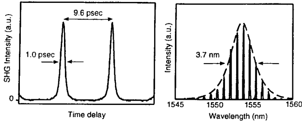
Figure 3. Autocorrelation trace and corresponding spectrum ( indicating theoretical spectral shape of \text{sech}^2 profile ) of 104 GHz repetition rate pulses generated using the nonlinear beat conversion technique in a step like dispersion profiled fibre.
