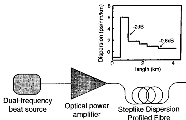
Figure 2. Schematic of the experimental configuration used to examine nonlinear beat signal conversion in a step like dispersion profiled fibre. Inset shows the actual step dispersion profile of the fibre employed.
