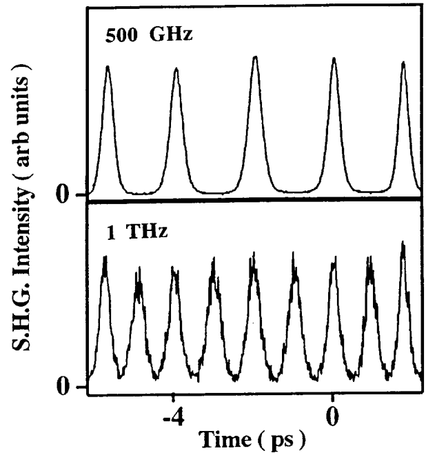
Figure 7. Autocorrelation traces of 500 GHz and 1 THz pulsetrains, generated using polarisation multiplexing.
