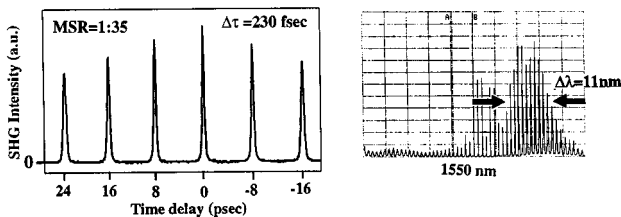
Figure 6. Autocorrelation trace of 230 fs solitons at 125 GHz repetition rate obtained via beat conversion in association with self frequency shifting techniques. The complementary 11 nm halfwidth spectrum (5 nm/div) can be seen distinct from the input carrier around 1555 nm.
