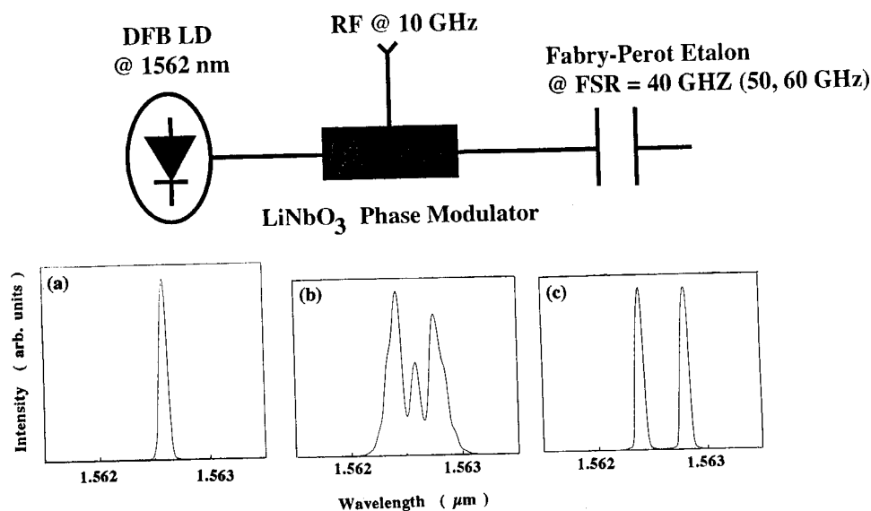
Figure 8. Schematic of sideband extraction configuration and related spectra.
