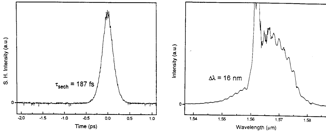
Figure 10. Autocorrelation trace of femtosecond pulses and their corresponding spectrum generated using the non linear conversion of dispersion compensated pulses from an electroabsorption modulator source at 10 GHz repetition rate.
