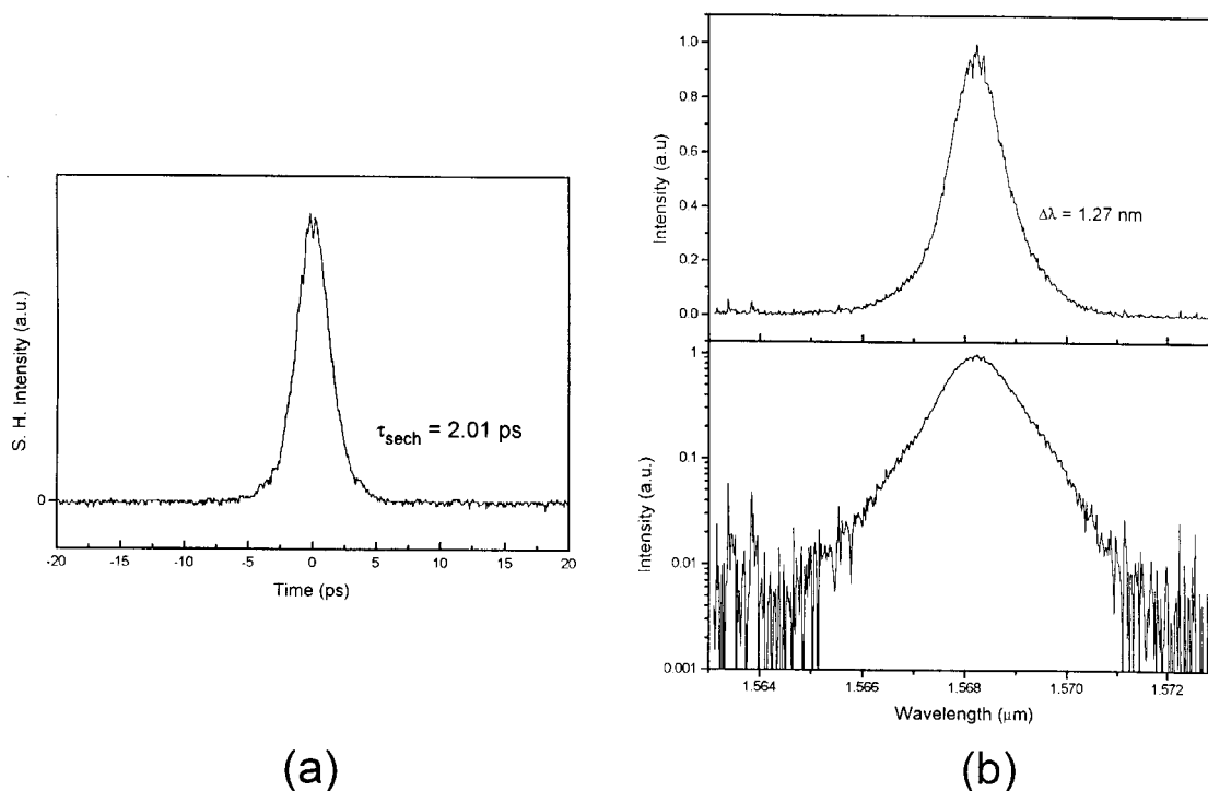
Figure 11. Autocorrelation trace and spectrum of tunable, picosecond 10 GHz pulses extracted from femtosecond soliton spectrum (see Fig. 10).
