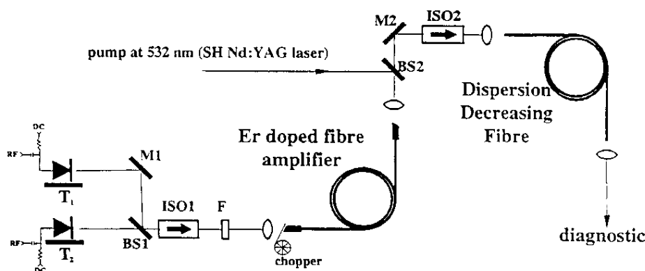
Figure 1. Schematic of original experimental configuration, employing dispersion decreasing fibre for high repetition rate soliton generation using laser diode nonlinear beat signal conversion.
